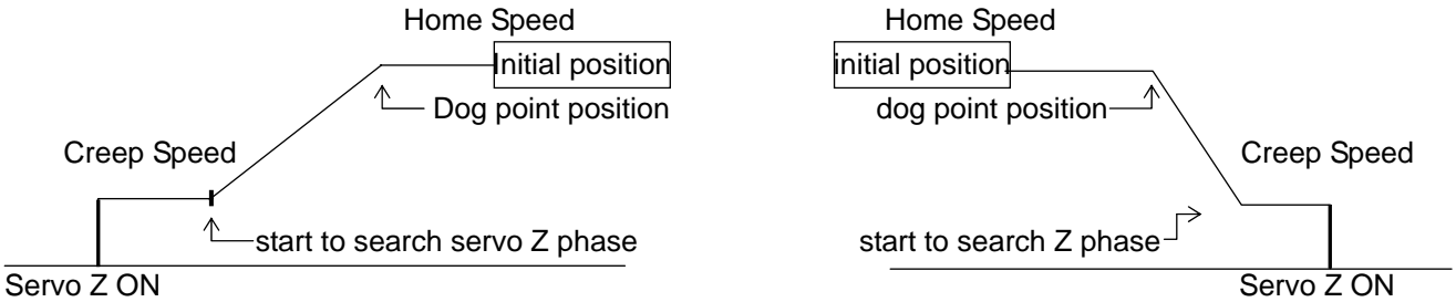
(2) reverse mode (when M8158=1 or M8159=1, Don't Care M8156 and M8157)
